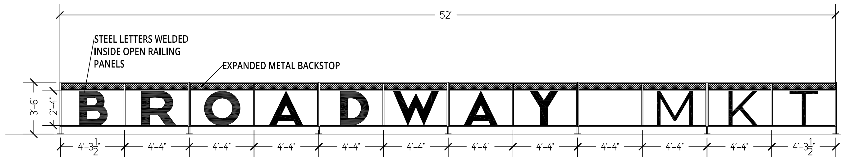
1 PATIO RAILING ELEVATION Scale: 1/4" = 1'-0"
